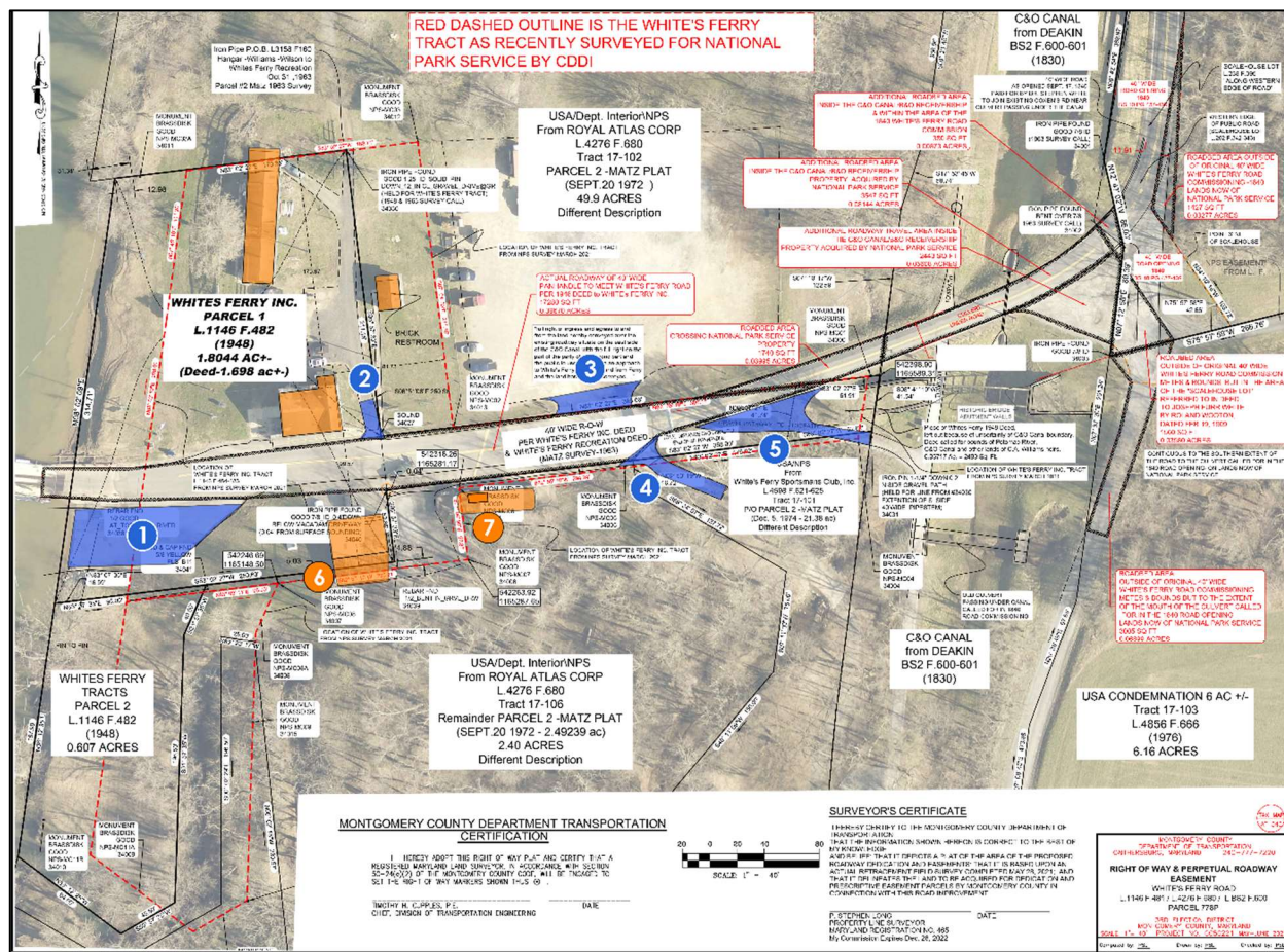
Figure 3-22: Official Survey of Maryland Side Lands
