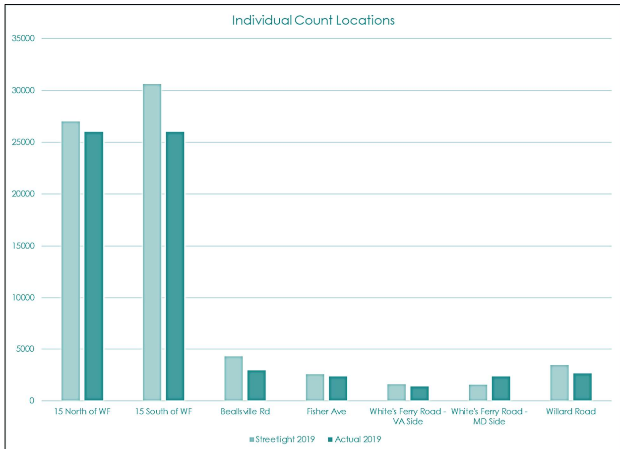
Figure 3-5: Comparison of Estimated and Observed Traffic Counts at Specific Locations
